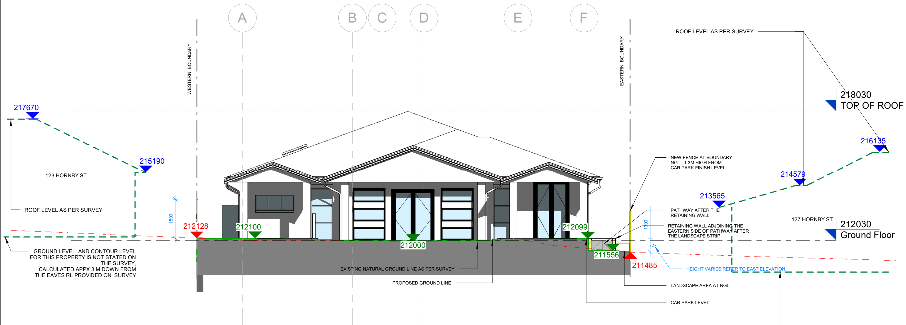
1 SECTION C - Cross Section Through Parking Number 4 & 14 1 : 100
